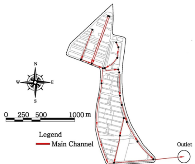
Fig. 3 The layout of main urban drainage channels
